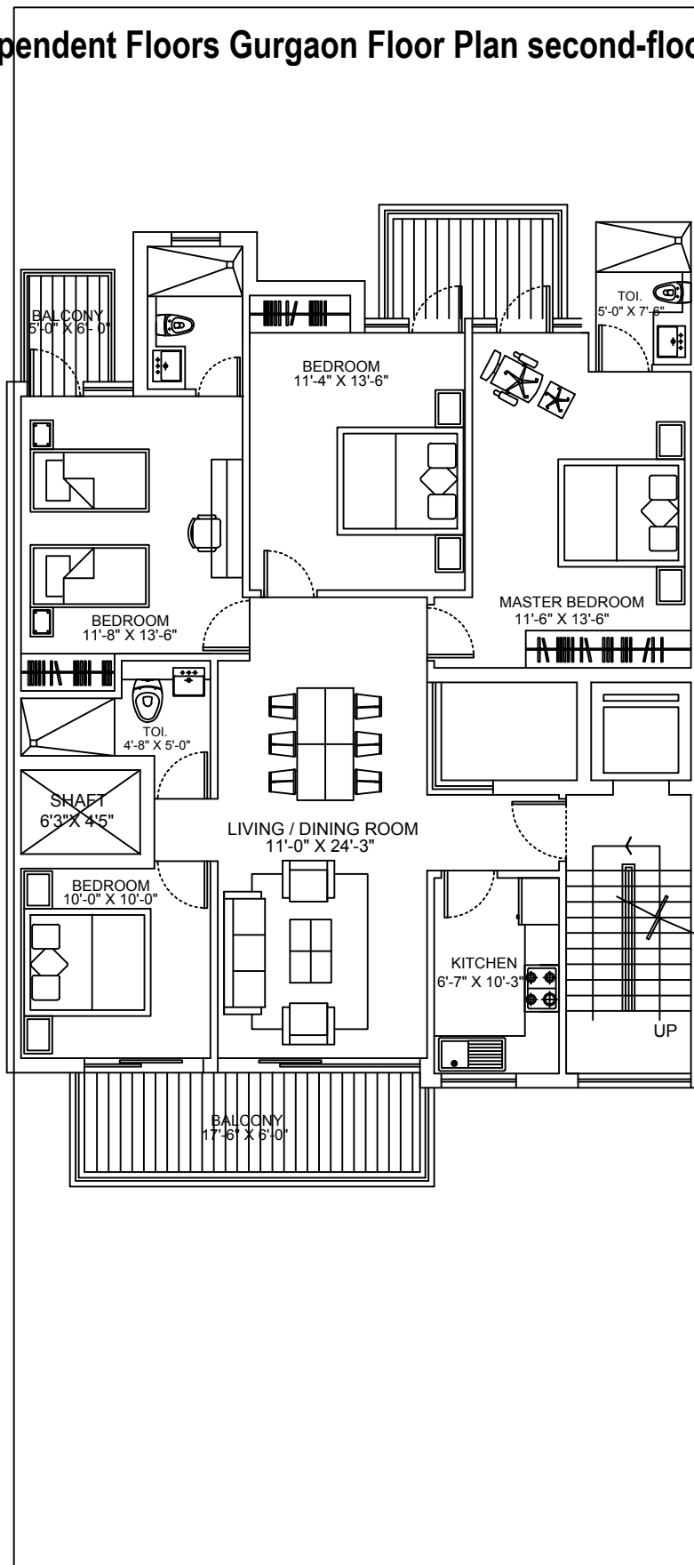
SECOND FLOOR
